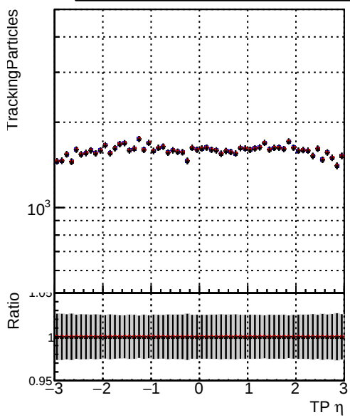
Legend: DQM_mkFit_baseline (blue line), DQM_mkFit_baseline6iter (red line), DQM_mkFit_TT_RetrainV2_WP1_6iter_ep3 (black line)
