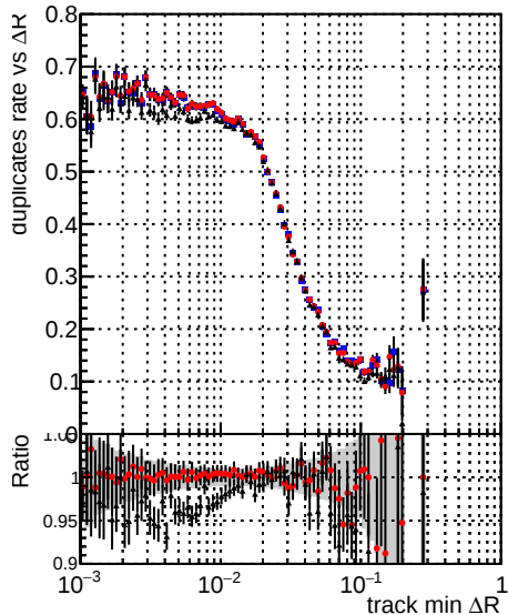
Legend: - \Delta R mkFit baseline - \Delta R mkFit baseline6iter - \Delta R mkFit TT_RetrainV2_WP1_6iter_ep3
