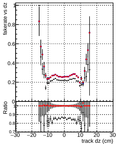
Fake rate vs dz DOM mkFit baseline DOM mkFit baselineGiter WP1 6iter ep3
