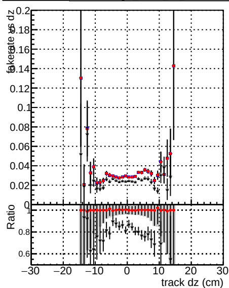
—•— DOM mkFit baseline —•— DOM mkFit baselineGitter —•— DOM mkFit TT RetrainV2 WP1 6iter ep3
