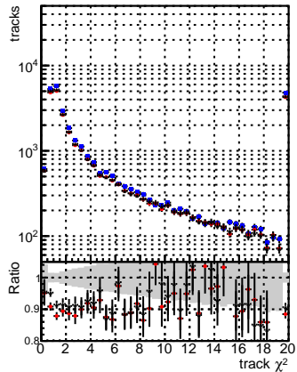
N of reco track vs. \chi^2 for DQM mFit baseline, DQM mFit 6iter, and DQM mFit WP1 6iter ep3
