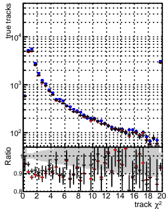
N of reco track vs. \chi^2 for DQM mFit baseline, DQM mFit 6iter, and DQM mFit WP1 6iter ep3
