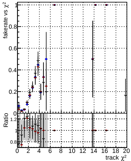
Fake rate vs. DOM mkFit baseline DOM mkFit baseline6iter DOM mkFit RetrainV2 WP1 6iter ep3
