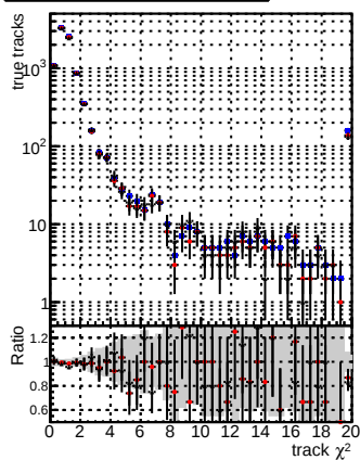
N of reco track vs. \chi^2 DOM mFit baseline DOM mFit+RetrainV2 DOM mFit+RetrainV2 WP1 6iter ep3
