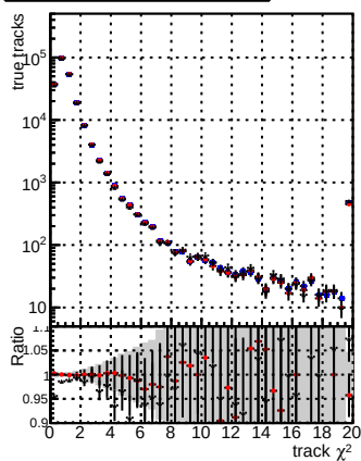
N of reco track vs. \chi^2 for WP1 6iter ep3
