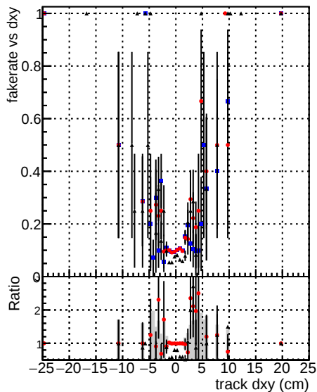
— DOM mkFit baseline — DOM mkFit baseline 6iter — DOM mkFit baseline 6iter WP1 — DOM mkFit baseline 6iter ep3
