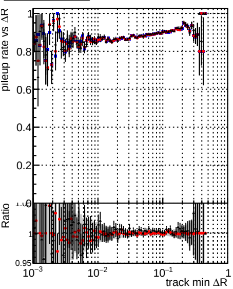
Legend: DQM_mkFit_baseline (black line with error bars), DQM_mkFit_baseline6iter (red line with error bars), DQM_mkFit_TT_RetrainV2_WP1_6iter_ep3 (black line with error bars)
