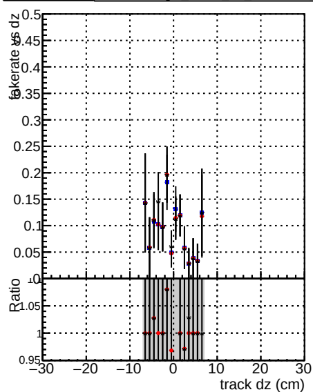
Fake rate vs dz Legend: DOM mkFit baseline DOM mkFit baselineGitter DOM mkFit TT RetrainV2 WP1 6iter ep3
