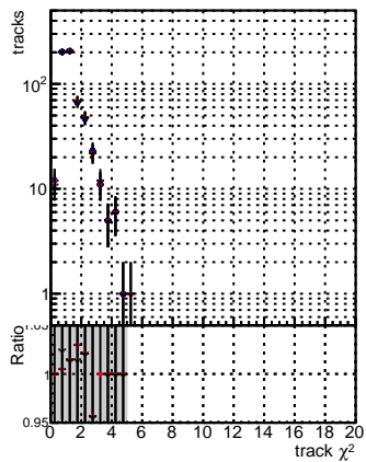
N of reco track vs. \chi^2 DGM mkFit baseline DGM mkFit baseline gitter DGM mkFit V1 Retrain V2 WP1 6iter ep3
