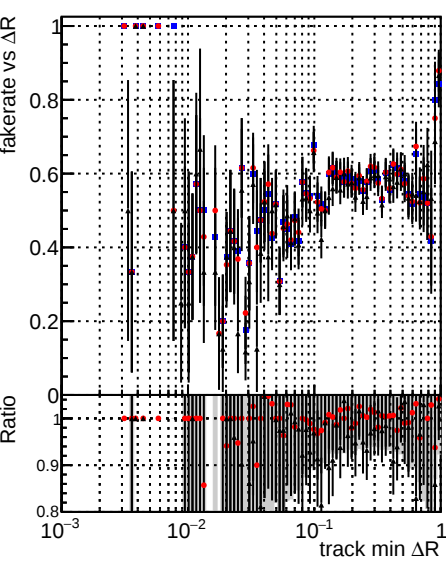
Legend: DQM_mkFit_baseline (black line with blue dots), DQM_mkFit_baseline6iter (red line with red dots), DQM_mkFit_TT_RetrainV2_WP1_6iter_ep3 (black line with black dots)
