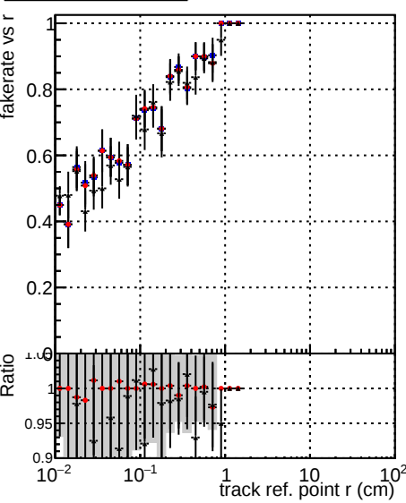
Legend: —●— DOM_mkFit_baseline —●— DOM_mkFit_baseline6iter —●— DOM_mkFit_TT_RetrainV2_WP1_6iter_ep3
