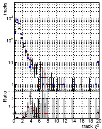
N of reco track vs. \chi^2 DGM mFit baseline DGM mFit baseline giter DGM mFit RetrainV2 WP1 6iter ep3
