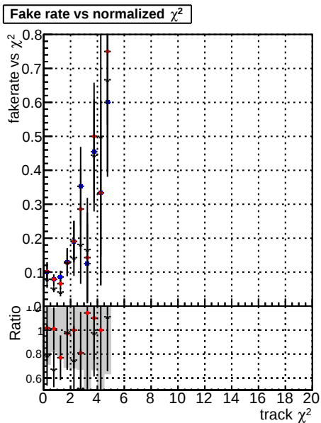
Fake rate vs. Legend: DOM mkFit baseline (blue circles), DOM mkFit baseline 6iter (red circles), DOM mkFit 11 RetrainV2 WP1 6iter ep3 (black circles)
