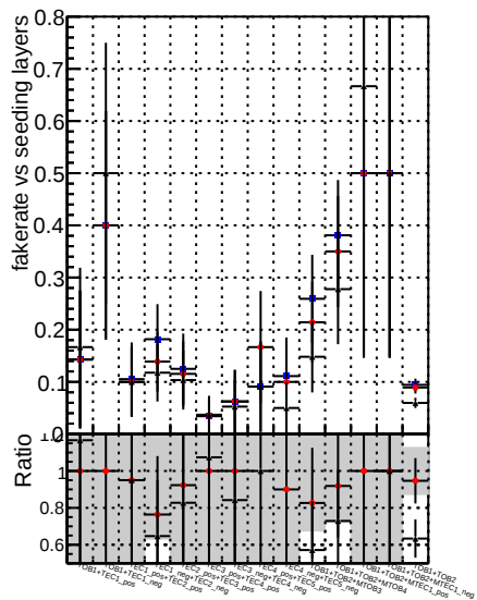
Fake rate vs. Legend: DOM mkFit baseline (blue circles), DOM mkFit baseline 6iter (red circles), DOM mkFit 11 RetrainV2 WP1 6iter ep3 (black circles)
