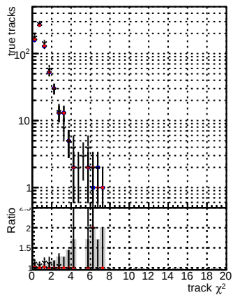
N of reco track vs. \chi^2 DQM mkFit baseline DQM mkFit baseline+gitter DQM mkFit V1+RetrainV2 WP1_6iter_ep3
