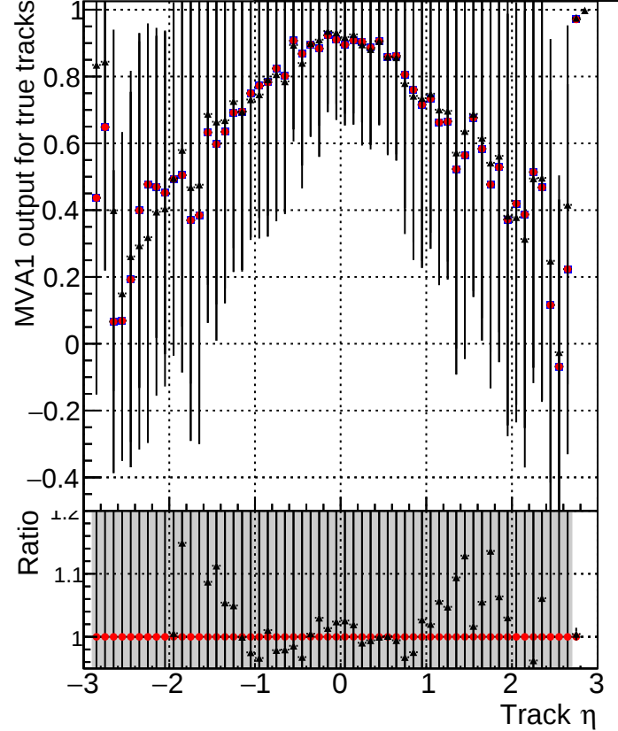
MVA1 of associated tracks (recoToSim) vs. track \eta Legend: ■ DQM_mkFit_baseline ● DQM_mkFit_baseline6iter ▲ DQM_mkFit_TT_RetrainV2_WP1_6iter_ep3
