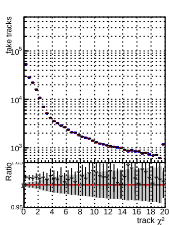
DOM mkFit baseline DOM mkFit baseline gitter DOM mkFit V1 Retrain V2 WP1 6iter ep3 overSet
