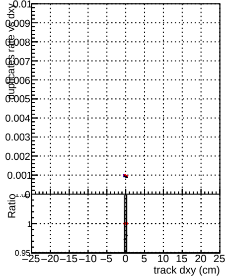
Duplicates Rate vs Dxy WP1 6iter ep3
