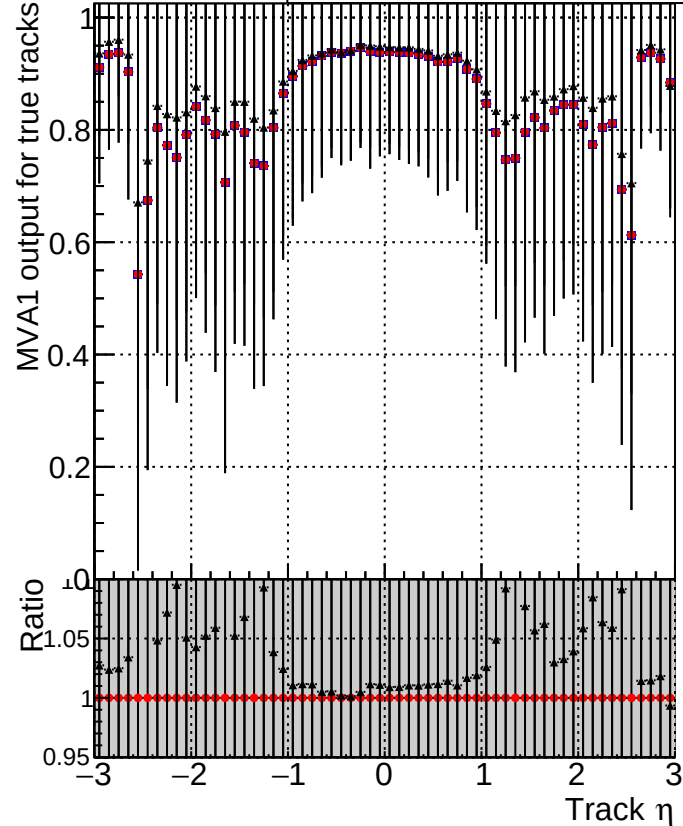
MVA1 of associated tracks (recoToSim) vs. track \eta Legend: ■ DQM_mkFit_baseline ● DQM_mkFit_baseline6iter ▲ DQM_mkFit_TT_RetrainV2_WP1_6iter_ep3
