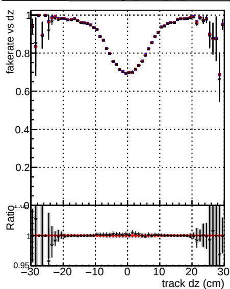
DOM mkFit baseline DOM mkFit baselineGitter DOM mkFit 11 RetrainV2 WP1 6iter ep3
