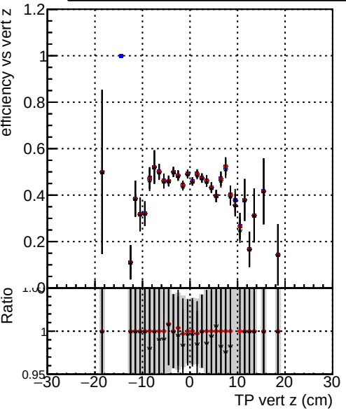
Efficiency vs TP vert z (cm) Legend: DQM_mkFit_baseline (blue line) DQM_mkFit_baseline6iter (red line) DQM_mkFit_TT_RetrainV2_WP1_6iter_ep3 (black line)
