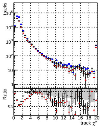
N of reco track vs. \chi^2 DOM mkFit baseline DOM mkFit DOM mkFit Retrain V2 WP1 6iter ep3
