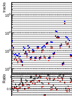
N of reco track vs. \chi^2 DOM mkFit baseline DOM mkFit DOM mkFit Retrain V2 WP1 6iter ep3
