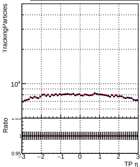
Legend: DQM_mkFit_baseline (blue line with circles) DQM_mkFit_baseline6iter (red line with circles) DQM_mkFit_TT_RetrainV2_WP1_6iter_ep3 (black line with circles)
