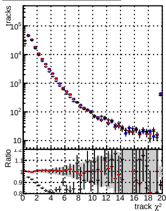
N of reco track vs. \chi^2 DOM mkFit baseline DOM mkFit baseline gitter DOM mkFit V2 Retrain WP1 6iter ep3
