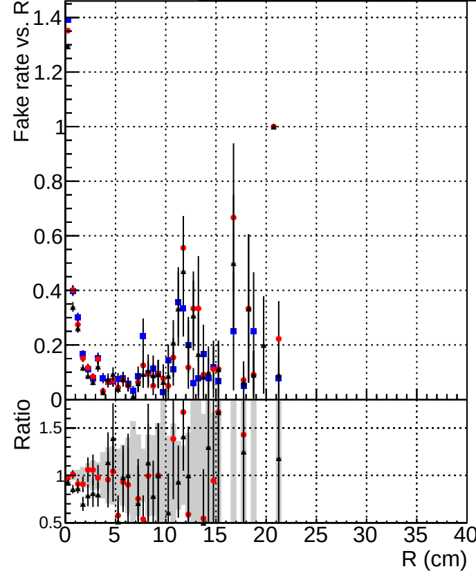
K_S^0 tracking fake rate vs R Legend: DQM_mkFit_baseline (blue squares) DQM_mkFit_baseline6iter (red circles) DQM_mkFit_TT_RetrainV2_WP1_6iter_ep3 (black triangles)
