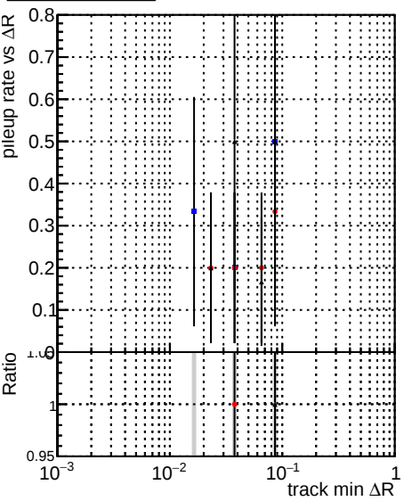
Legend: DQM_mkFit_baseline (blue dot), DQM_mkFit_baseline6iter (red dot), DQM_mkFit_TT_RetrainV2_WP1_6iter_ep3 (black dot)
