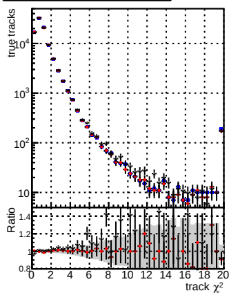
N of reco track vs. \chi^2 DOM mkFit baseline DOM mkFit baseline gitter DOM mkFit V2 WP1 6iter ep3
