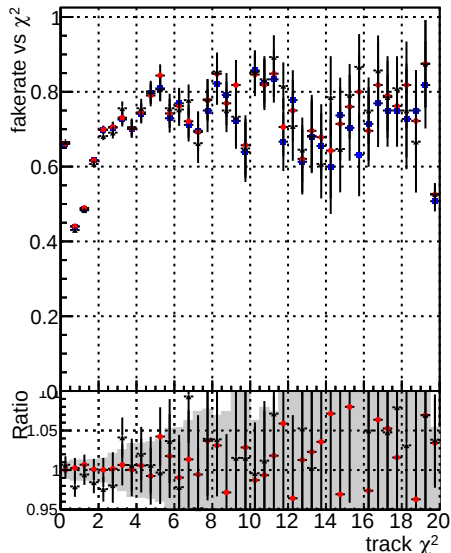
Fake rate vs. DOM mkFit baseline DOM mkFit baseline6iter DOM mkFit RetrainV2 DOM mkFit WP1 6iter ep3
