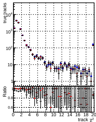
N of reco track vs. \chi^2 — baseline — mFit — mFit+gitter WP1 6iter ep3
