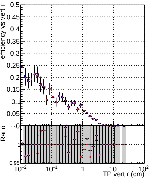
Efficiency vs vertpos Legend: DOM mkFit5 XiMinusNOPU base DOM mkFit5 XiMinusNOPU retrainOldFiles125_v2_prelimWPM_epoch4 DOM mkFit6 XiMinusNOPU base DOM mkFit6 XiMinusNOPU retrainOldFiles125_v2_prelimWPM_epoch4 DOM mkFit5 XiMinusNOPU retrainOldFiles125_v2_ANDPLessRetrain_epoch4
