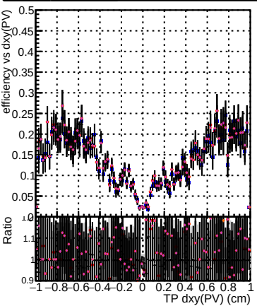
Efficiency vs Dxy(PV) Legend: DOM_mkFit5_XiMinusNOPU_base DOM_mkFit5_XiMinusNOPU_retrainOldFiles125_v2_prelimWPM_epoch4 DOM_mkFit6_XiMinusNOPU_base DOM_mkFit6_XiMinusNOPU_retrainOldFiles125_v2_prelimWPM_epoch4 DOM_mkFit5_XiMinusNOPU_retrainOldFiles125_v2_ANDPLessRetrain_epoch4
