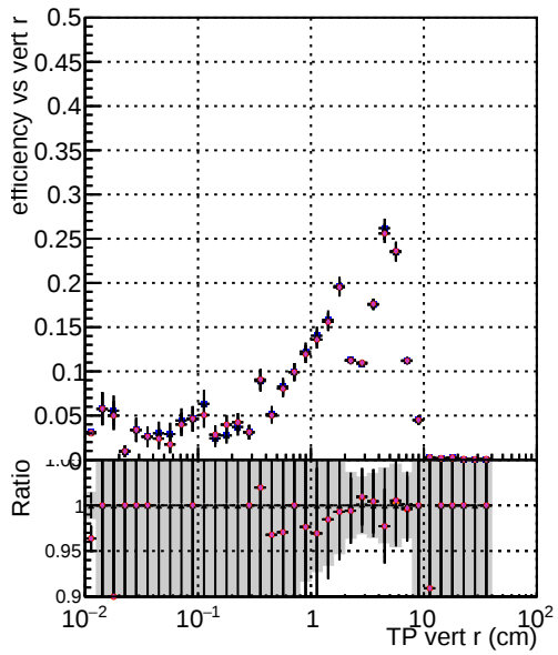
Efficiency vs vertpos Legend: DOM mkFit5 XiMinusNOPU base DOM mkFit5 XiMinusNOPU retrainOldFiles125_v2_prelimWPM_epoch4 DOM mkFit5 XiMinusNOPU base DOM mkFit6 XiMinusNOPU retrainOldFiles125_v2_prelimWPM_epoch4 DOM mkFit5 XiMinusNOPU retrainOldFiles125_v2_ANDPLessRetrain_epoch4
