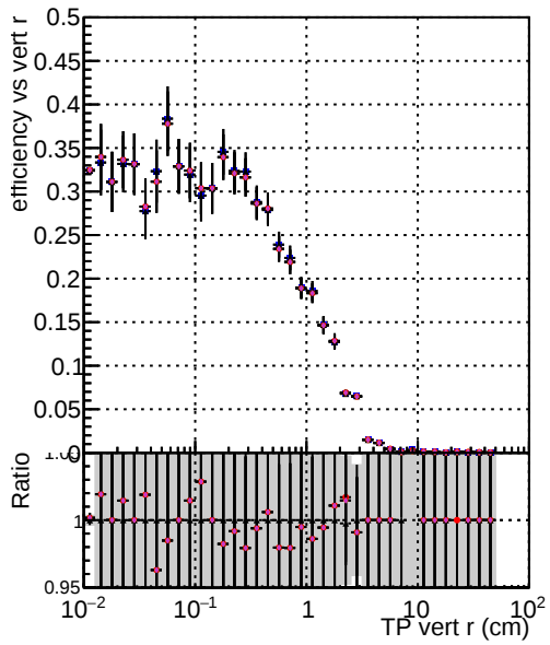
Efficiency vs vertpos Legend: DOM mkFit5 XiMinusNOPU base DOM mkFit5 XiMinusNOPU retrainOldFiles125_v2_prelimWPM_epoch4 DOM mkFit6 XiMinusNOPU base DOM mkFit6 XiMinusNOPU retrainOldFiles125_v2_prelimWPM_epoch4 DOM mkFit5 XiMinusNOPU retrainOldFiles125_v2_ANDPLessRetrain_epoch4
