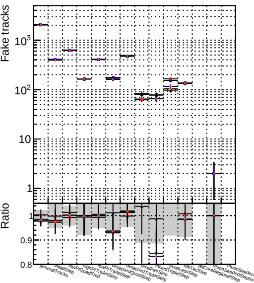
Numbe Model Configuration 1 DOM mkFit6 XiMinusNOPU base 2 DOM mkFit6 XiMinusNOPU retrainOldFiles125 v2 prelimWPM epoch4 3 DOM mkFit5 XiMinusNOPU retrainOldFiles125 v2 ANDPLessRetrain epoch4
