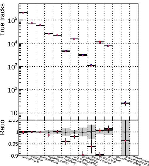
DOM mkFit5 XiMinusNOPU base DOM mkFit5 XiMinusNOPU retrainOldFiles125 v2 prelimWPM epoch4
