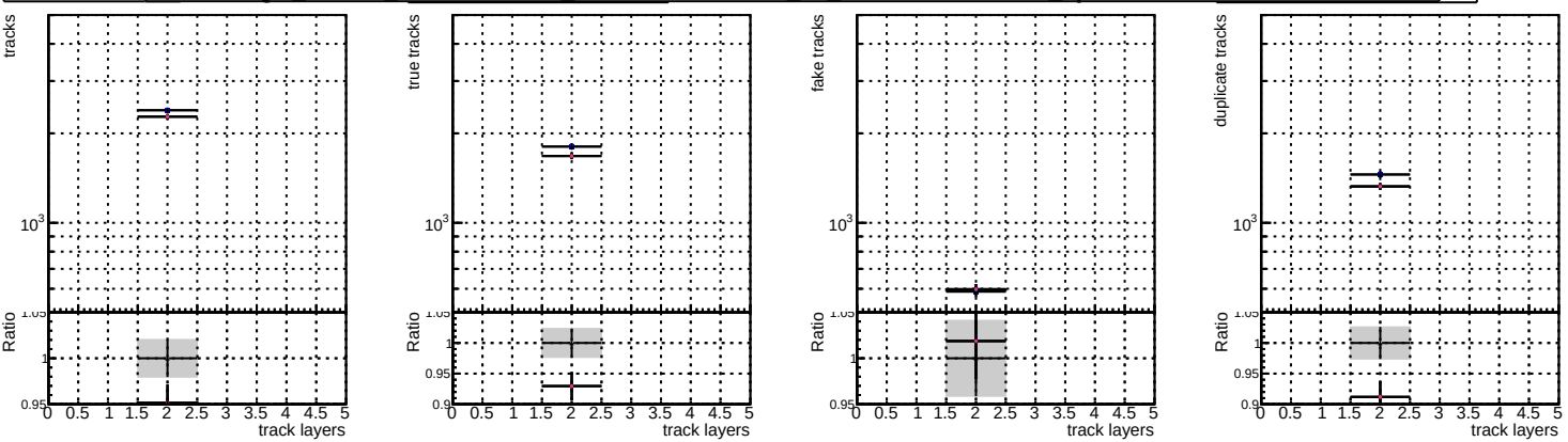
N of reco track vs hit N of associated (recoToSim) tracks vs hit fake tracks N of associated (recoToSim) duplicate tracks vs hit base train oldFiles v2
