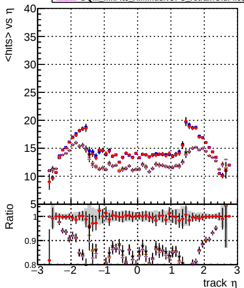
mean hits vs \eta DOM mkFit5 XMinusNOPU_retrainOldFiles125_v2_prelimWPM_epoch4 DOM mkFit5 XMinusNOPU_base DOM mkFit6 XMinusNOPU_retrainOldFiles125_v2_prelimWPM_epoch4 DOM mkFit5 XMinusNOPU_retrainOldFiles125_v2_ANDLessRetrain_epoch4
