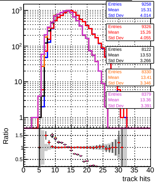
mean hits DOM mkFit5 XMinusNOPU_base DOM mkFit5 XMinusNOPU_retrainOldFiles125_v2_prelimWPM_epoch4 DOM mkFit5 XMinusNOPU_base DOM mkFit5 XMinusNOPU_retrainOldFiles125_v2_prelimWPM_epoch4 DOM mkFit5 XMinusNOPU_retrainOldFiles125_v2_ANDLessRetrain_epoch4
