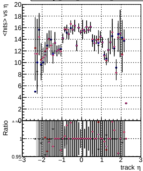
mean hits vs \eta DOM mkFit5 XiMinusNOPU_retrainOldFiles125_v2_prelimWPM_epoch4 DOM mkFit5 XiMinusNOPU_retrainOldFiles125_v2_prelimWPM_epoch4 DOM mkFit5 XiMinusNOPU_retrainOldFiles125_v2_prelimWPM_epoch4 DOM mkFit5 XiMinusNOPU_retrainOldFiles125_v2_ANDPlessRetrain_epoch4
