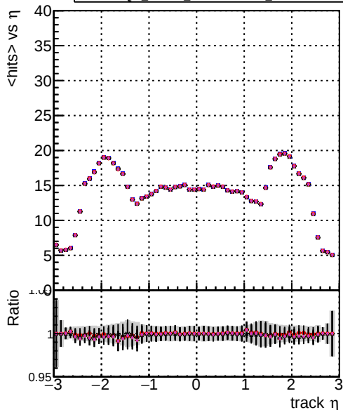
DOM mkFit5 XiMinusNOPU_base DOM mkFit5 XiMinusNOPU_retrainOldFiles125_v2_prelimWPM_epoch4 DOM mkFit6 XiMinusNOPU_base DOM mkFit6 XiMinusNOPU_retrainOldFiles125_v2_prelimWPM_epoch4 DOM mkFit5 XiMinusNOPU_retrainOldFiles125_v2_ANDLessRetrain_epoch4
