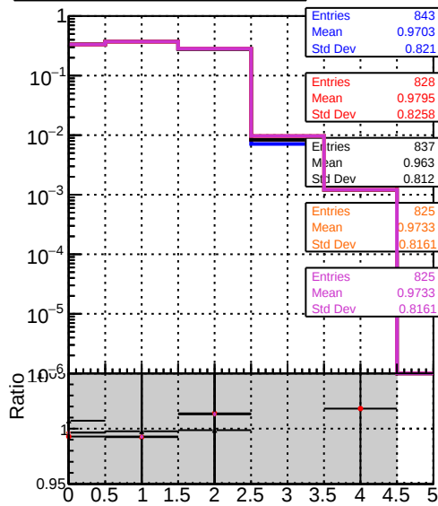
mean hits vs \eta DOM mkFit5 XiMinusNOPU_retrainOldFiles125_v2_prelimWPM_epoch4 DOM mkFit5 XiMinusNOPU_base DOM mkFit6 XiMinusNOPU_retrainOldFiles125_v2_prelimWPM_epoch4 DOM mkFit5 XiMinusNOPU_retrainOldFiles125_v2_ANDLessRetrain_epoch4
