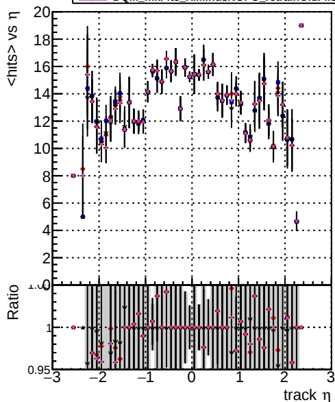
mean hits vs \eta DOM mkFit5 XiMinusNOPU_retrainOldFiles125_v2_prelimWPM_epoch4 DOM mkFit5 XiMinusNOPU_base DOM mkFit6 XiMinusNOPU_retrainOldFiles125_v2_prelimWPM_epoch4 DOM mkFit5 XiMinusNOPU_retrainOldFiles125_v2_ANDLessRetrain_epoch4
