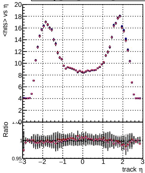
mean hits vs \eta DOM mkFit5 XiMinusNOPU base DOM mkFit5 XiMinusNOPU retrainOldFiles125_v2_prelimWPM_epoch4 DOM mkFit5 XiMinusNOPU base DOM mkFit5 XiMinusNOPU retrainOldFiles125_v2_prelimWPM_epoch4 DOM mkFit5 XiMinusNOPU retrainOldFiles125_v2_ANDPLeRefrain_epoch4
