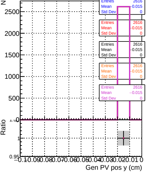
GeneratedAllV_Y DOM mkFit5 X Minus NOPU base DOM mkFit5 X Minus NOPU retrainOldFiles125_v2_prelimWPM_epoch4 DOM mkFit5 X Minus NOPU retrainOldFiles125_v2_prelimWPM_epoch4 DOM mkFit5 X Minus NOPU retrainOldFiles125_v2_ANDLessRetrain_epoch4
