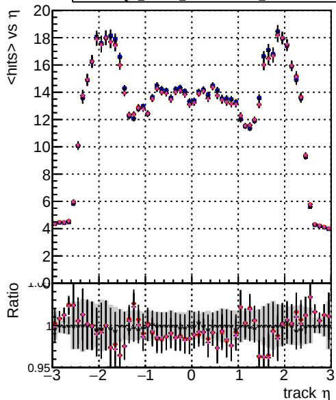
mean hit DOM mkFit5 XiMinusNOPU_retrainOldFiles125_v2_prelimWPM_epoch4 DOM mkFit5 XiMinusNOPU_base DOM mkFit6 XiMinusNOPU_retrainOldFiles125_v2_prelimWPM_epoch4 DOM mkFit5 XiMinusNOPU_retrainOldFiles125_v2_ANDLessRetrain_epoch4
