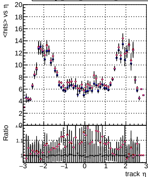
mean hits vs \eta Legend: DOM mkFit5 XMinusNOPU_retrainOldFiles125_v2_prelimWPM_epoch4 (blue), DOM mkFit5 XMinusNOPU_retrainOldFiles125_v2_prelimWPM_epoch4 (red), DOM mkFit5 XMinusNOPU_retrainOldFiles125_v2_prelimWPM_epoch4 (orange), DOM mkFit5 XMinusNOPU_retrainOldFiles125_v2_prelimWPM_epoch4 (purple)
