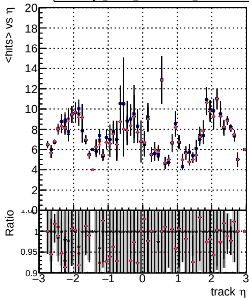
mean hit DOM mkFit5 XMinusNOPU retrainOldFiles125_v2_prelimWPM_epoch4 DOM mkFit5 XMinusNOPU retrainOldFiles125_v2_prelimWPM_epoch4 DOM mkFit5 XMinusNOPU retrainOldFiles125_v2_prelimWPM_epoch4 DOM mkFit5 XMinusNOPU retrainOldFiles125_v2_prelimWPM_epoch4
