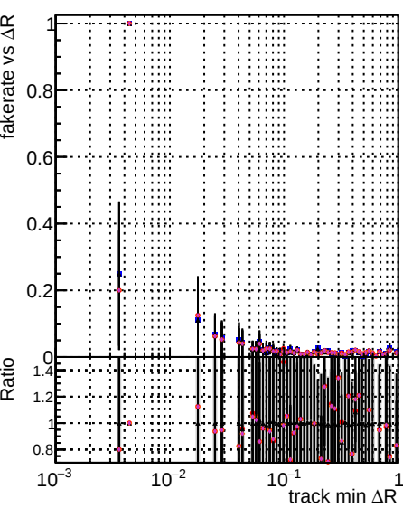
Fake rate vs \Delta R(\text{track, jet}) for RetrainOldFiles125_v2_prelimWPM_epoch4, RetrainOldFiles125_v2_prelimWPM_epoch4, RetrainOldFiles125_v2_ANDLessRetrain_epoch4, and RetrainOldFiles125_v2_prelimWPM_epoch4
