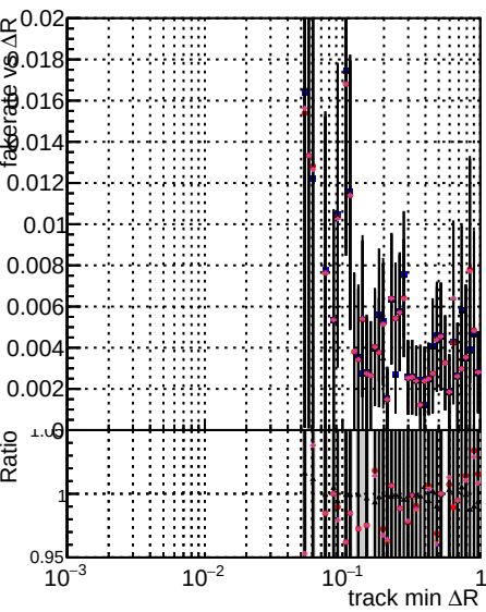
Fake rate vs \Delta R(\text{track, jet}) for RetrainOldFiles125 v2 AND LessRetrain epoch4
