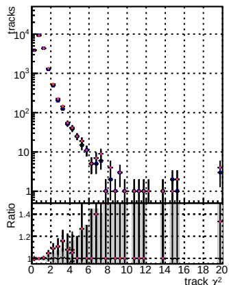
N of reco track vs. \chi^2 for different datasets and epochs
